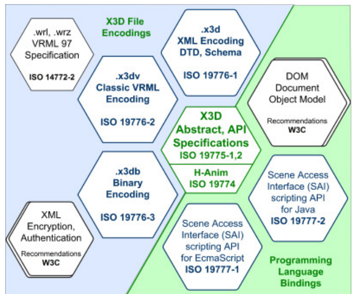
Figure 6: The ISO-IEC family of X3D standards.
