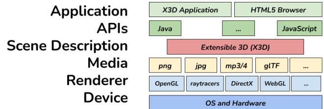
Figure 3: Example X3D Applications stack from a media-type perspective
