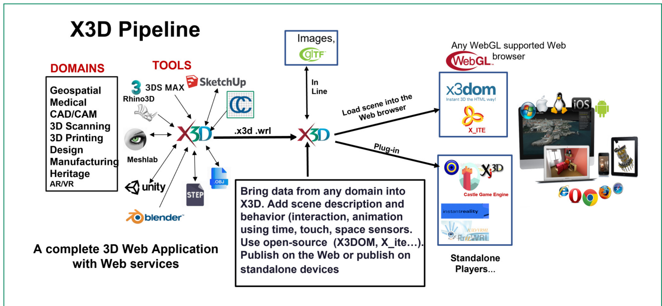
Figure 4: X3D functional support for the publishing ecosystem
